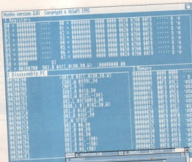
The MonAm debugger in all its glory
